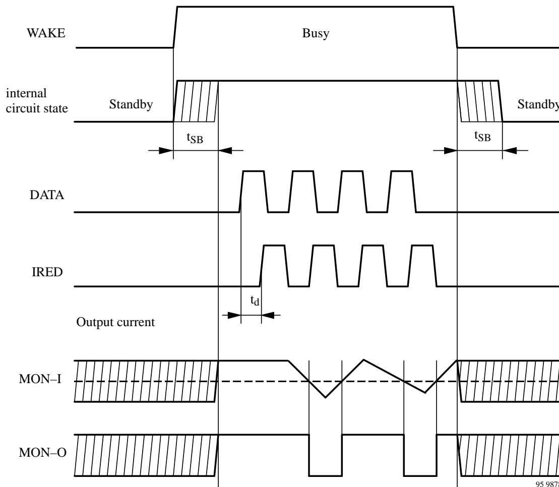
Figure 3. Timing diagram
